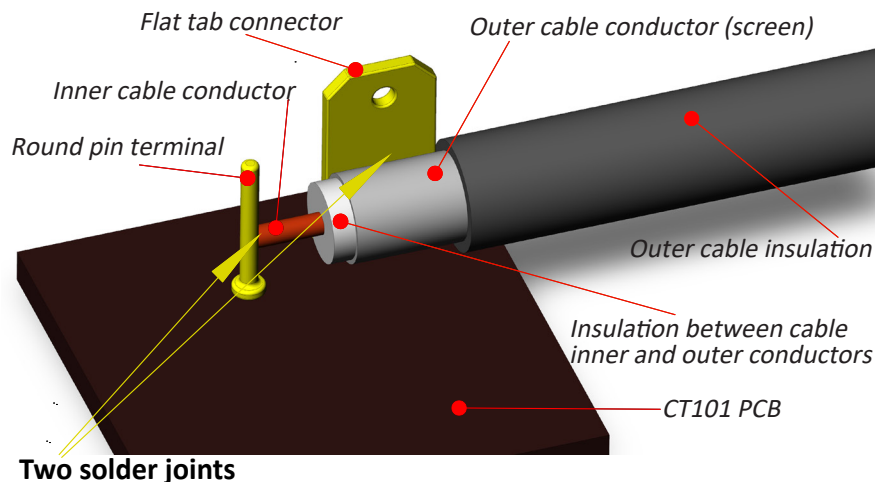
Fig. 3. CT101 audio signal input/output connections
