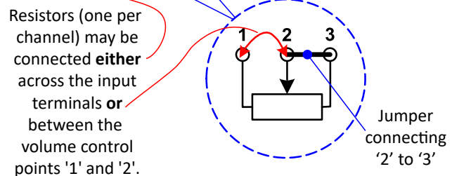
Fig. 8. Using CT101 without volume control but with resistors controlling the input resistance
