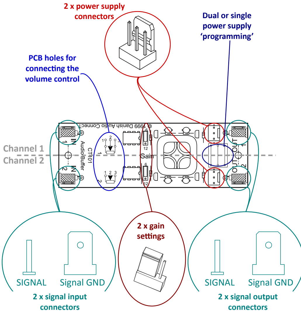
Fig. 1. CT101 connections
