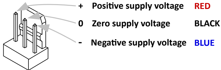
Fig. 2. CT101 power supply connections
