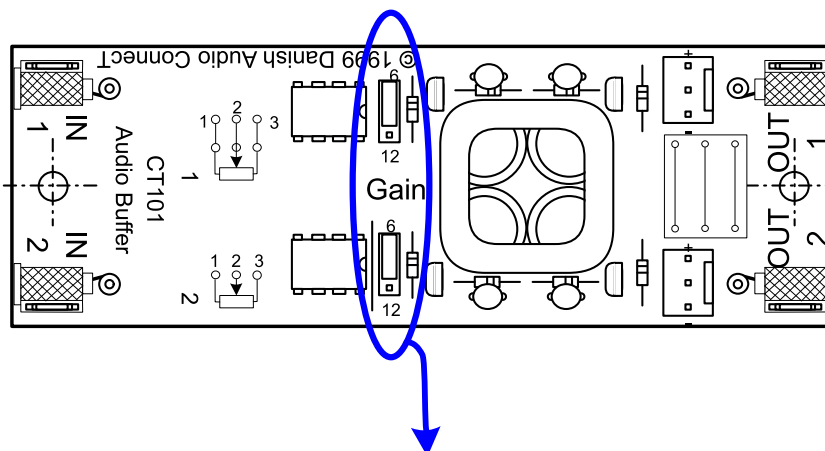
Fig. 9. CT101 gain settings
