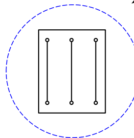
Using one power supply for each channel: The jumpers are not mounted
